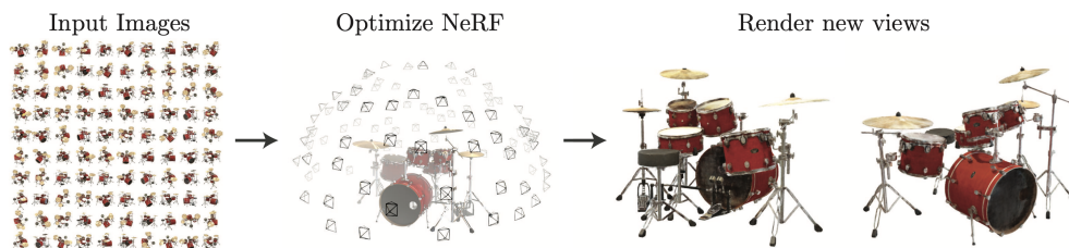
Figure 4.7: NeRF-based Reconstruction. Adapted from [2]. Given a set of input images with known camera poses, the NeRF model is optimized to produce novel views of the object. A similar pipeline is followed for the majority of NeRF-based methods presented in this section.
