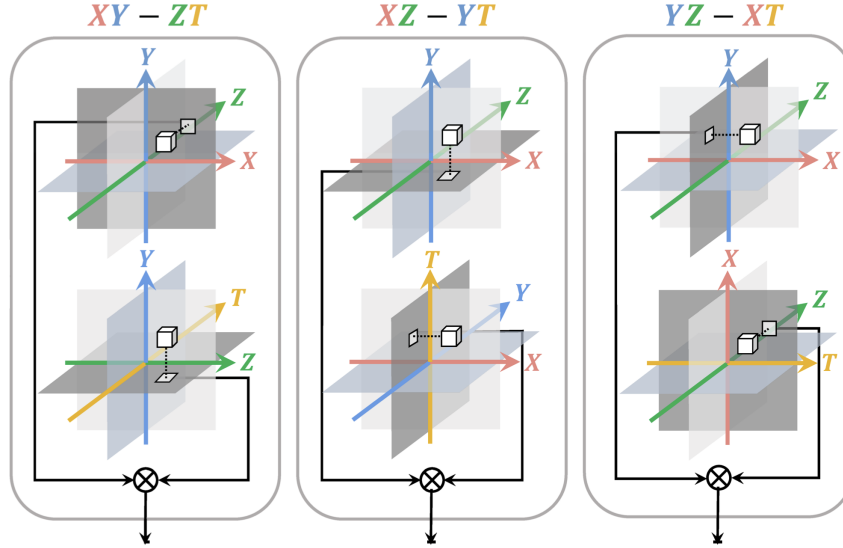
Figure 4.6: HexPlanes for Dynamic Reconstruction. Adapted from [46]. HexPlane proposes to parameterize dynamic 3D scenes into 6 planes of learnable features in 3D space, which are then concatenated at the end as input to a tiny MLP.
