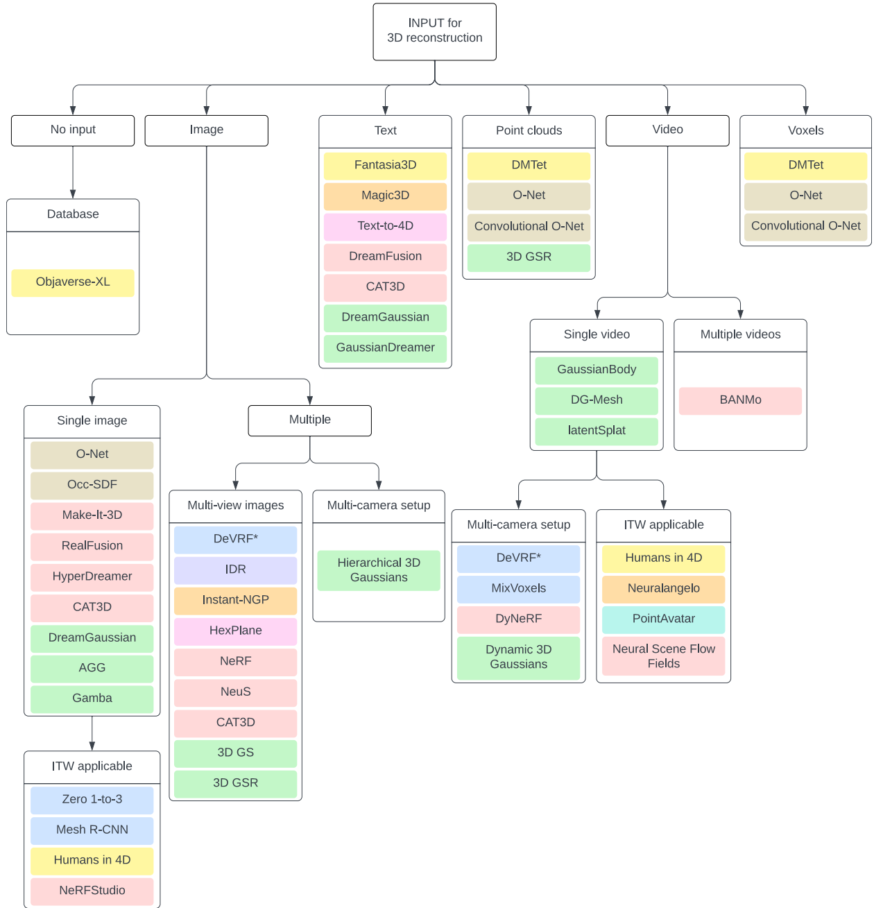
Figure 5.1: Input-based Taxonomy. The input-based categorization is a classic taxonomy structuring. Approaches with multiple input types are replicated under their respective input branches. Titles marked with an asterisk (*) indicate that the method requires input consisting of all other input types the title is categorized under.
