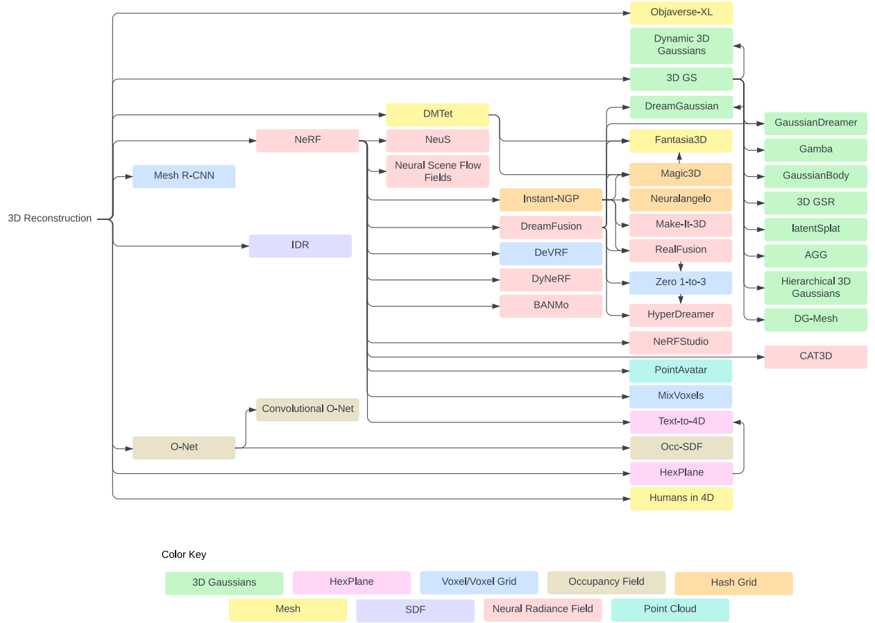
Figure 4.1: Literature Overview. A visualization of all literature reviewed for this thesis. Tree column 1 indicates 2019, column 2 indicates 2020, and so on until 2024. Arrows indicate direct or heavy influence. Node colors indicate its method’s main 3D representation, as shown in the legend at the bottom. For hybrid representations, we have chosen to categorize using the most prevalent representation.
