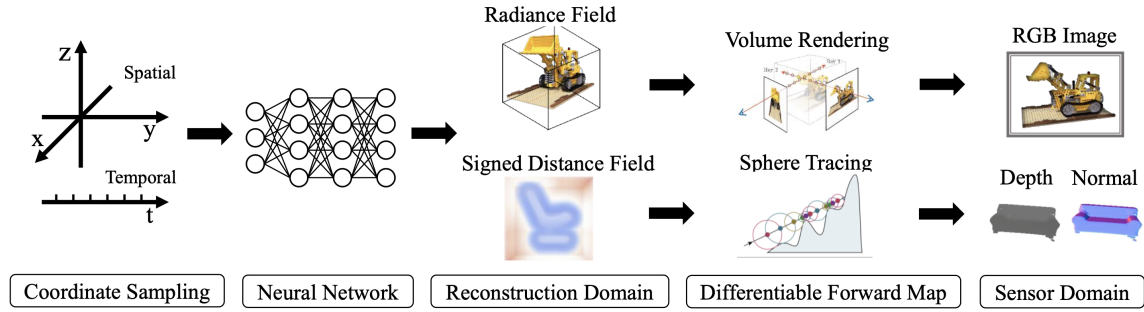
Figure 3.7: Neural Fields. Figure 3 (adapted [2], [27]) from Xie et al. [8]. Adapted for this thesis.
