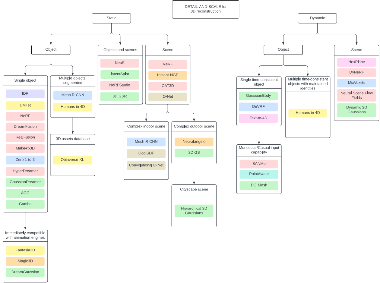
Figure 5.3: Scale-based Taxonomy. The scale-based taxonomy is rooted in the methods’ suitability in scale of reconstruction. We separate the methods into static and dynamic reconstruction scale and sort each tree individually. The ordering from least to most complex/large in scale is obtained with a top-down depth-first search prioritizing leftmost nodes on each tree, respectively.
