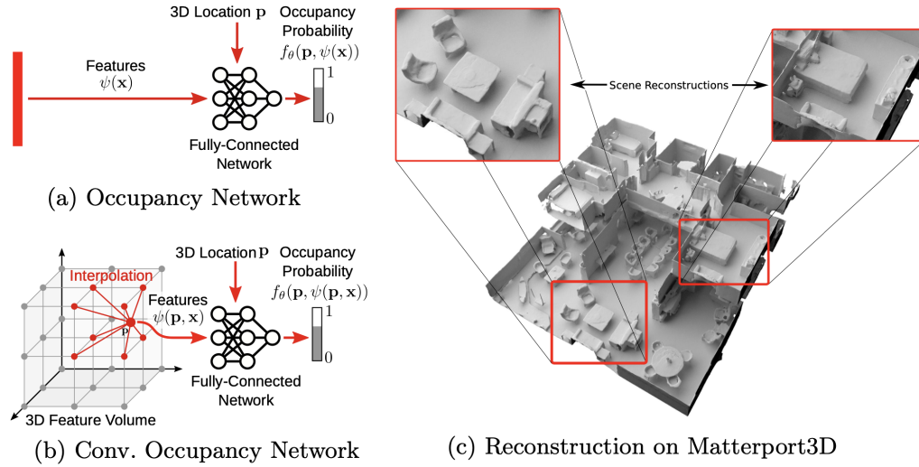
Figure 4.4: ONet-based Reconstruction. Figure 1 from [42] depicting the difference between a) the occupancy network approach and that of b) the convolutional o-net approach with c) the resulting complex, large indoor scene reconstruction using convolutional occupancy networks.
