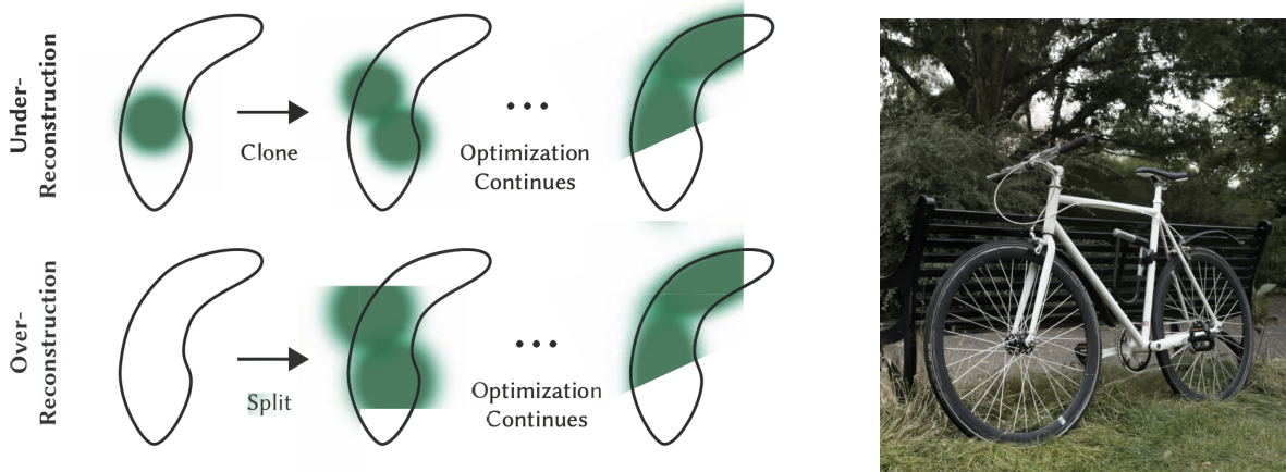
Figure 4.8: Gaussian-based Reconstruction. Figure (left) and result image (right) from [3]. The figure illustrates the Gaussian optimization method: if the Gaussian is too small, it is cloned (top), and if it is too large, it is split (bottom).
