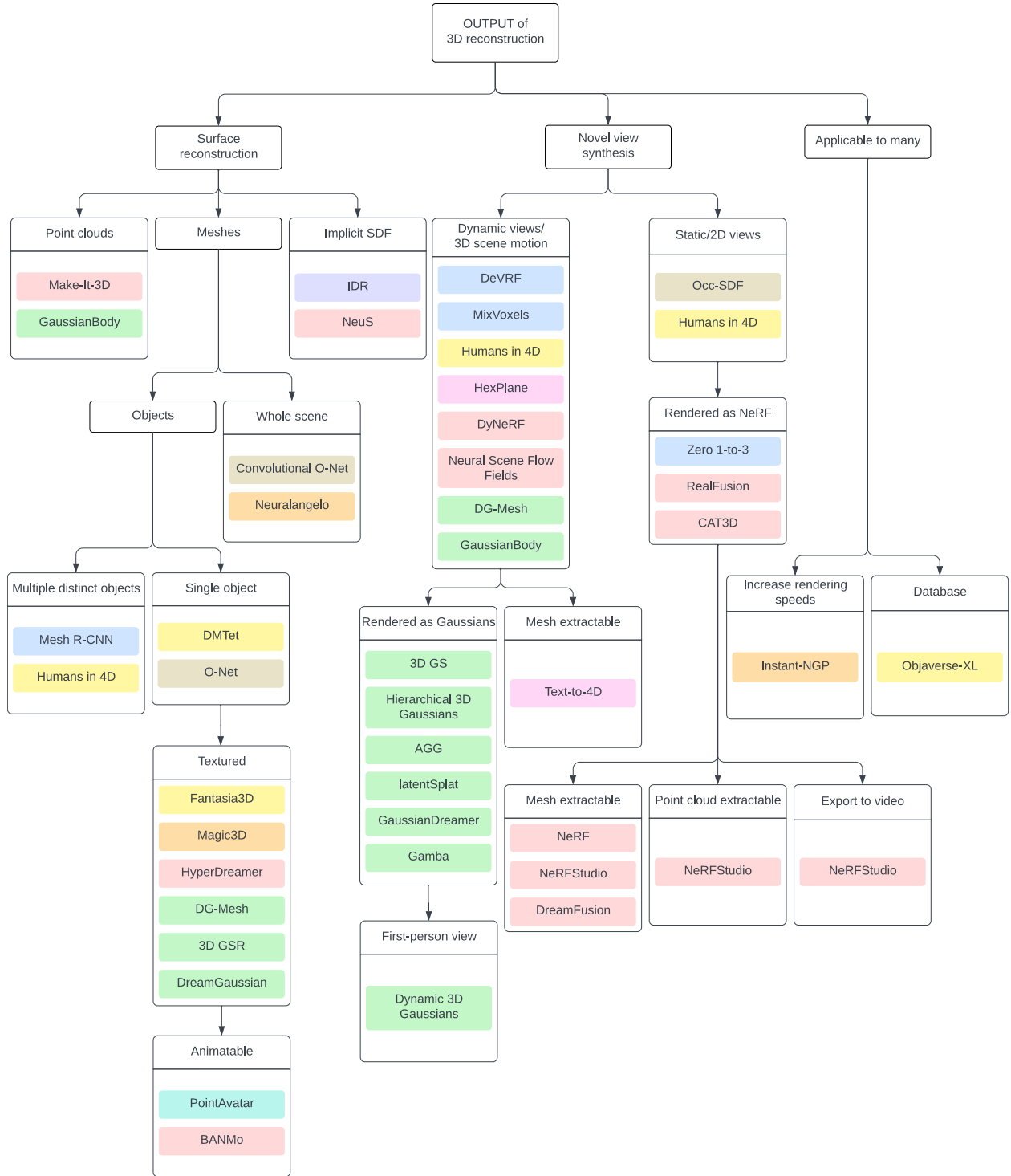
Figure 5.2: Output-based Taxonomy. The output-based taxonomy is first organized on the methods’ output goal and second on their respective output geometry representation. ‘Extractable’ primitive categories indicate the NVS methods whose results can further be processed with existing surface extraction algorithms to obtain the respective 3D geometry.
